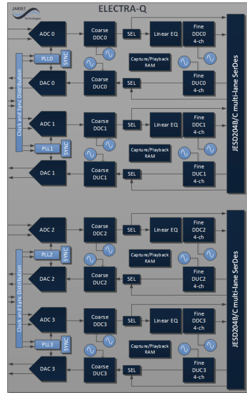
Electra-Q Block Diagram
